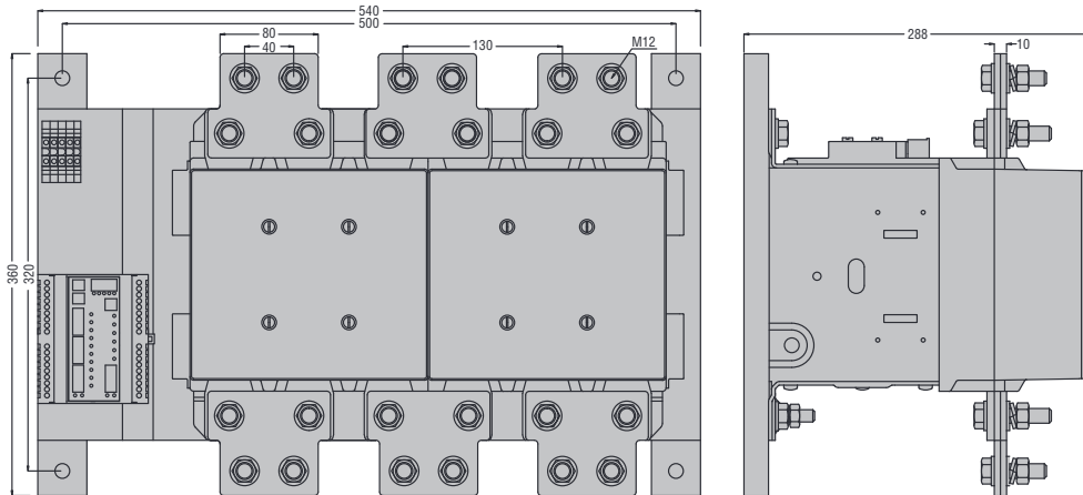
B1250 - B1600 3-polig
