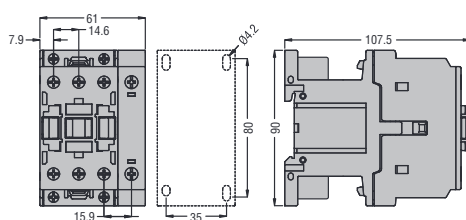
BF26T... - BF38T... D und L 4-polig
