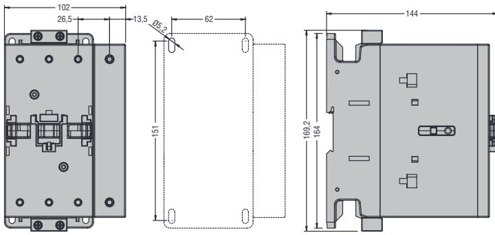
BF95T4A... - BF115T4A... - BF150T4A... 4-polig
