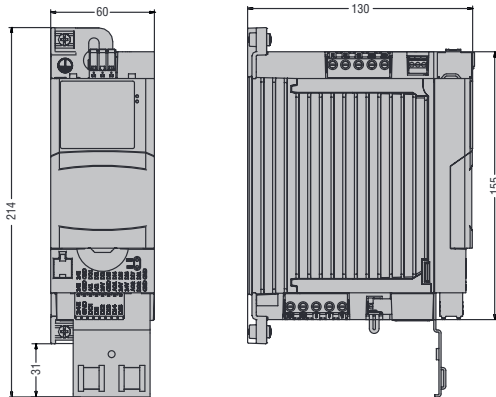
3-PHASIGE FREQUENZUMRICHTER VLB30004A480
