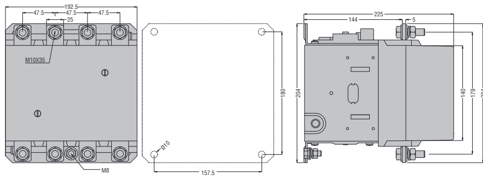
B2504 - B3104 - B4004 4-polig
