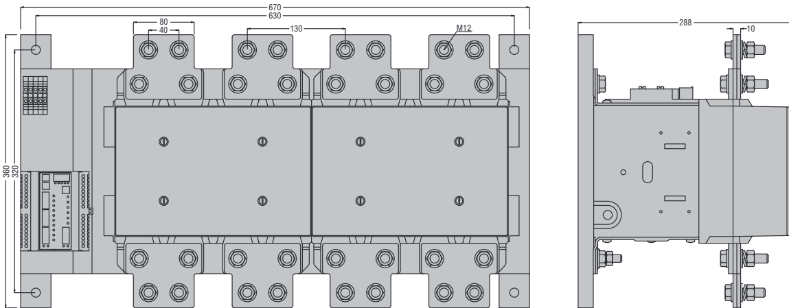
B12504 - B1600 4-polig
